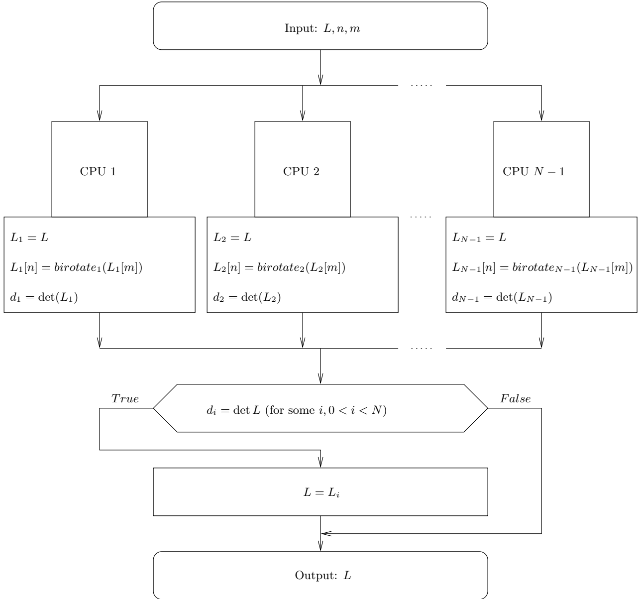
Figure 4.1: Schematic diagram representing the parallelized BIROT algorithm
